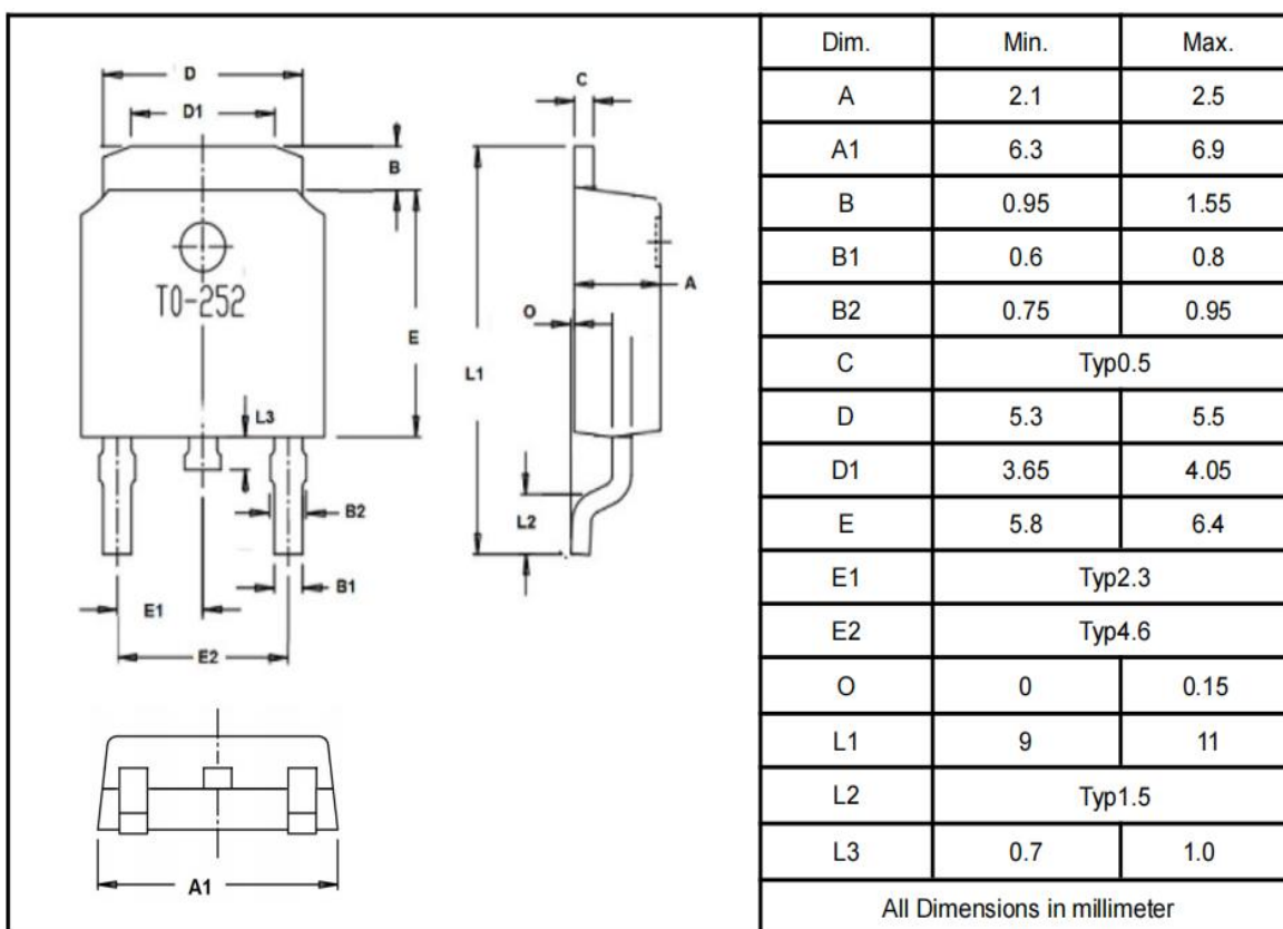
TO-252
