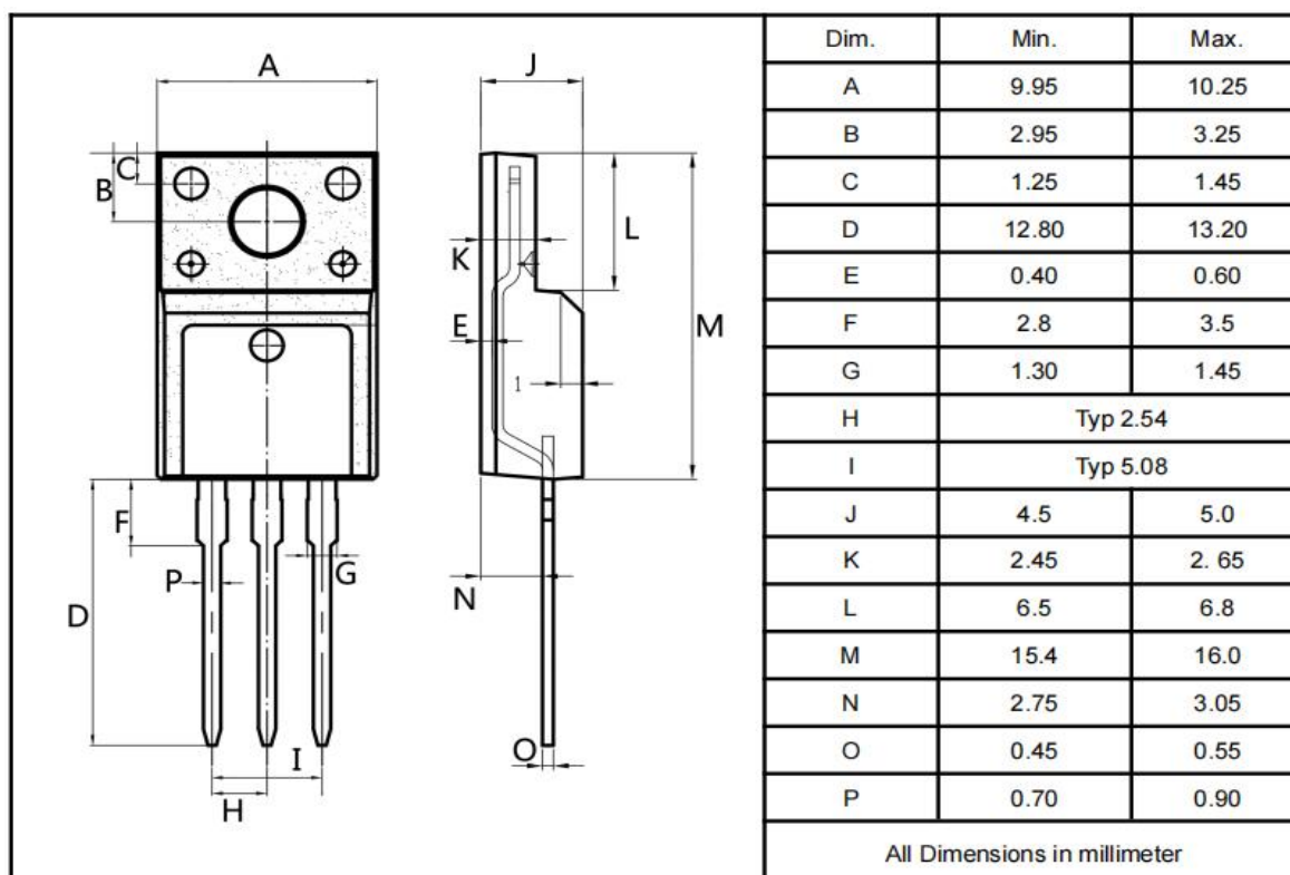
TO-220F
