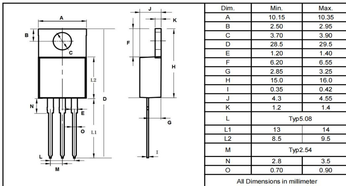
TO-220AB
